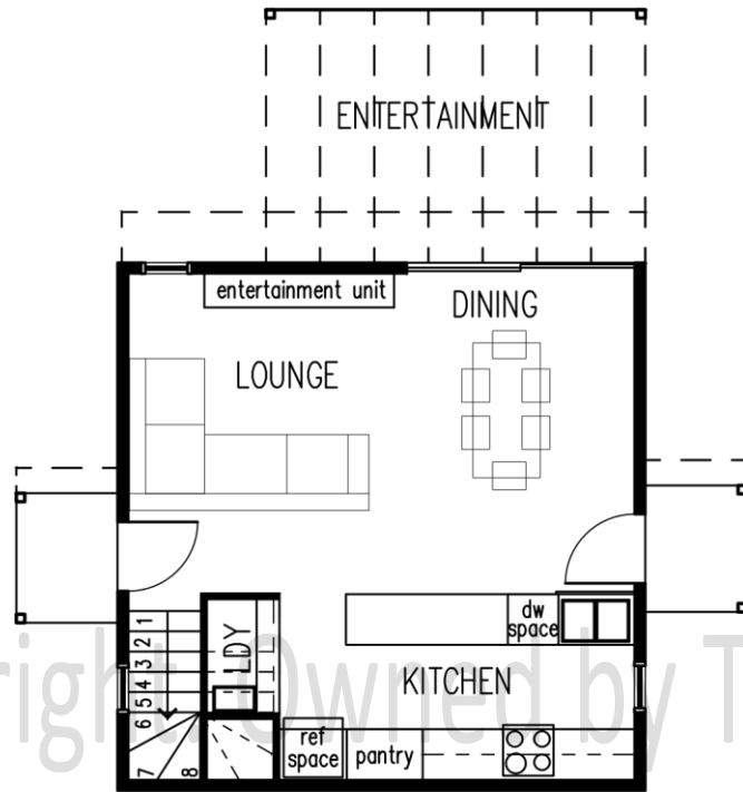
GROUND FLOOR internal floor area - 36m/sq
